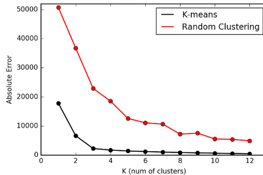
Figure 10.16: The error curve for k -means clustering on the point set of Figure 10.12 showing a bend in the elbow reflecting the three major clusters in the data. The error curve for random cluster centers is shown for comparison.
