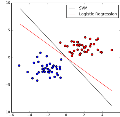
Figure 11.9: Both logistic regression and SVMs produce separating lines between point sets, but optimized for different criteria.
